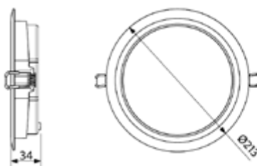
LEDDownlightRc-SI-E Rd200
