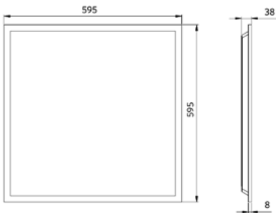
LEDPanelS-E4 Re295-32W
