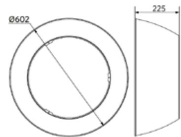
LEDHighbay-E2 Reflector-Rd602
