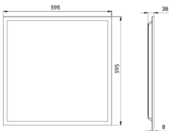
LEDPanelS-B3 Re295-32W
